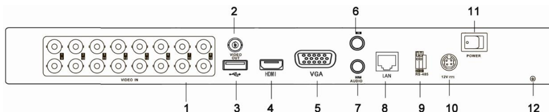
Figure 1.8 Rear Panel of DS-7216HFI-SH and DS-7216HWI-SH
